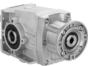
Aluminium helical bevel gearboxes 0.09kW to 5.5kW 20mm to 35mm shaft
