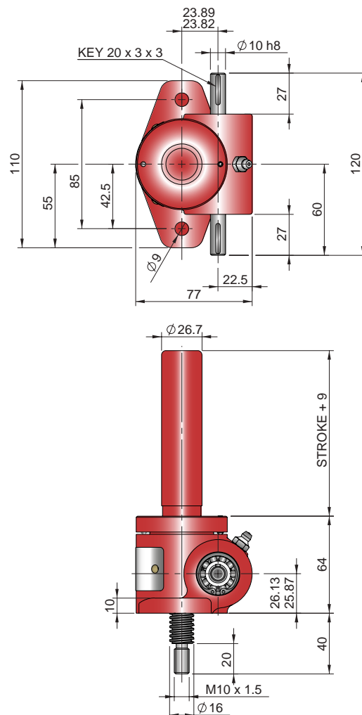
Inverted EMT0005-I00
