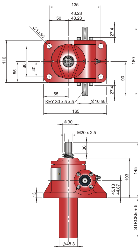
Upright EMT0025-U00
