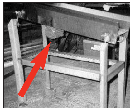
SPWT-80 on screen feeder.
