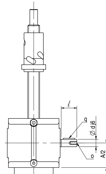
Vers.1: single input shaft
