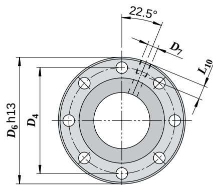
Flange type: 2 8 holes at 45° ( d_0 \geq 40 mm)
