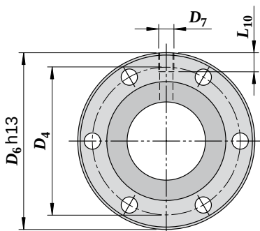
Flange type: 1 6 holes at 60° ( d_0 < 40 mm)
