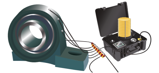
Direct lubrication of a bearing using combination of Easy Grease and hoseset.
